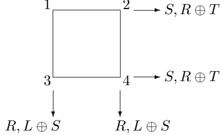
Figure 3: A representation of the 8 equations # in L, S, R, T .
